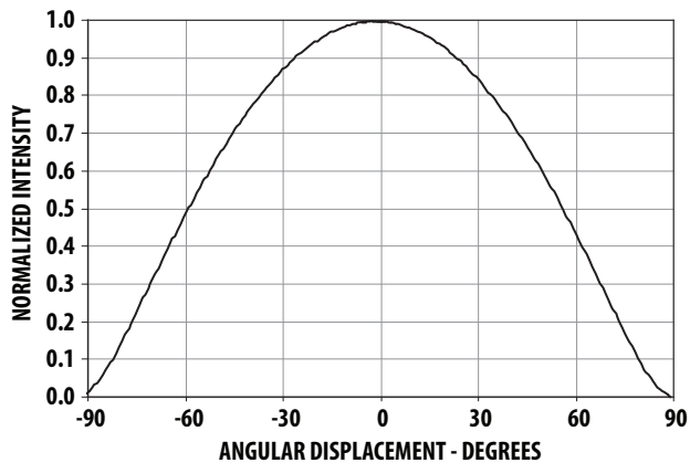
Figure 9. Radiation Pattern
