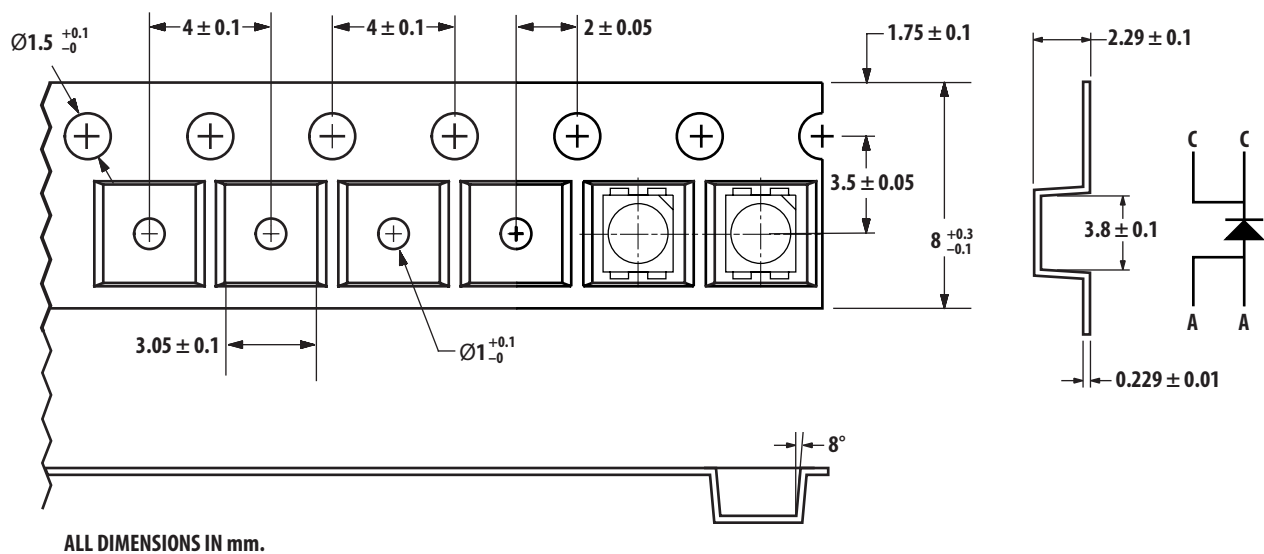
Figure 14. Tape Dimensions
